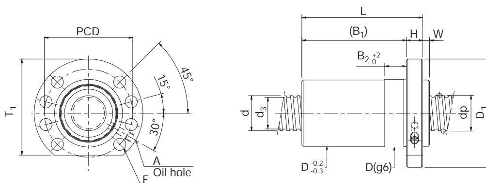
Drilling template 2
