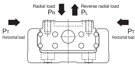
SKR: 4-way loads
